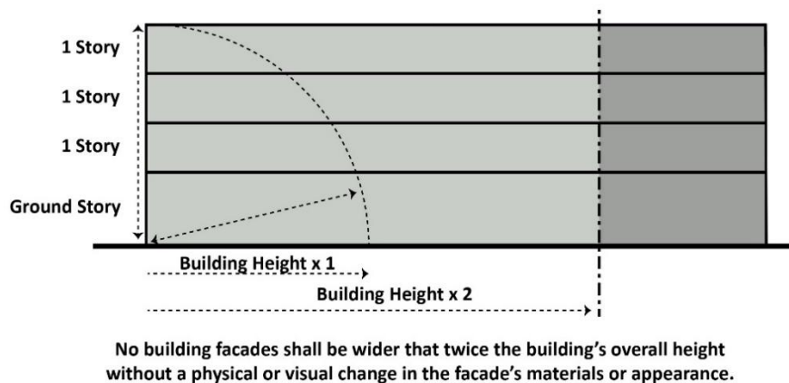
Figure 5: Maximum Façade Segment Length Measurement Example
